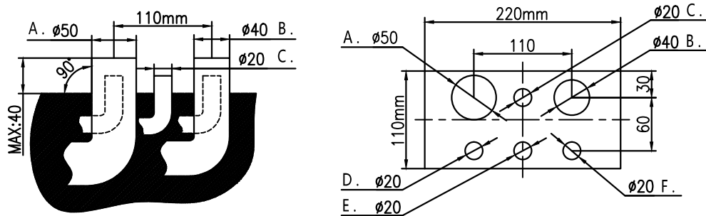
A .Waste pipe B .Suction tube D .Power input C .Water supply pipe E .Communication circuit F .Air source input
